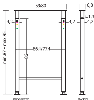
Gambone per penisola "TORN" regolabile Adjustable support for peninsula "TORN"
