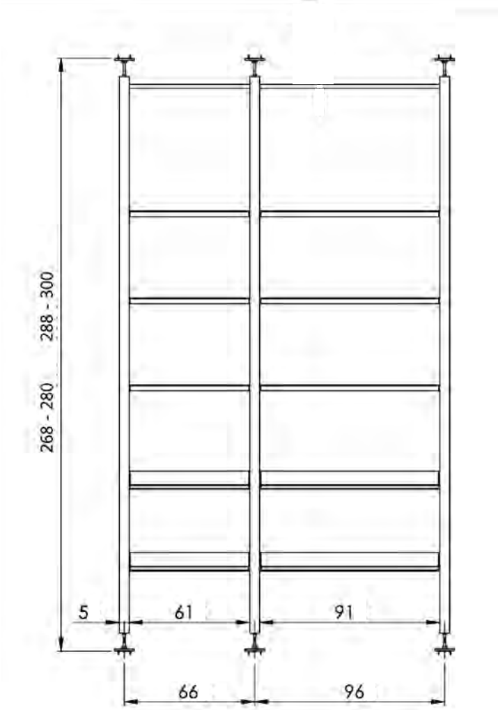
VISTA FRONTALE FRONT VIEW
