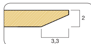
Profilo inclinato “LI” Inclined profile “LI”
