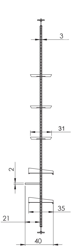
VISTA LATERALE SIDE VIEW
