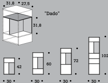
PENSILE A GIORNO "JUMPY" + "DADO" "JUMPY" + "DADO" OPEN WALL UNITS ÉLÉMENTS HAUTS SOSPENSUS OUVERTS "JUMPY" + "DADO" Verticale
