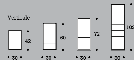
PENSILE A GIORNO "JUMPY" + "DADO" "JUMPY" + "DADO" OPEN WALL UNITS ÉLÉMENTS HAUTS SOSPENSUS OUVERTS "JUMPY" + "DADO" Verticale
