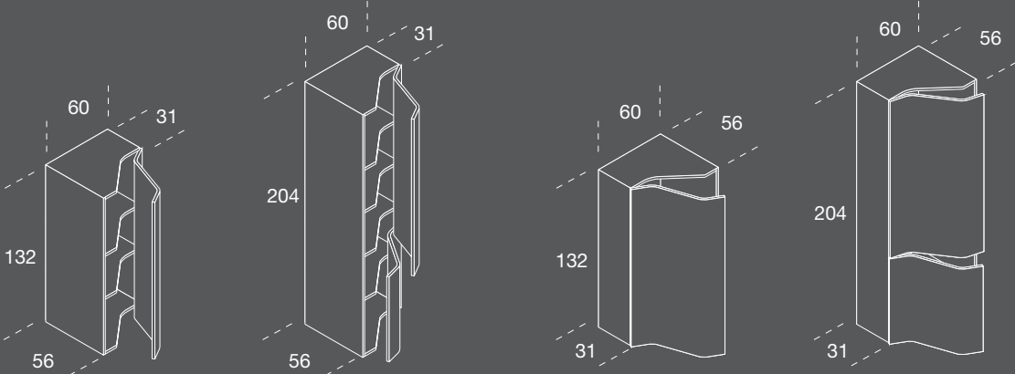
colonne h 132 cm e h 204 cm / apertura Dx e Sx column units h 132 cm and h 204 cm / RH and LH opening
