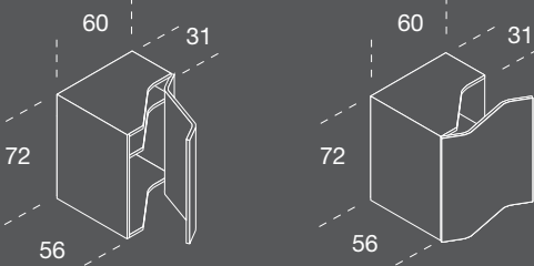
pensili da h 72 cm a h 96 cm / apertura Dx e Sx wall units from h 72 cm to h 96 cm / RH and LH opening
